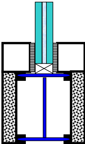
System Jansen Janisol thermally broken symmetric
